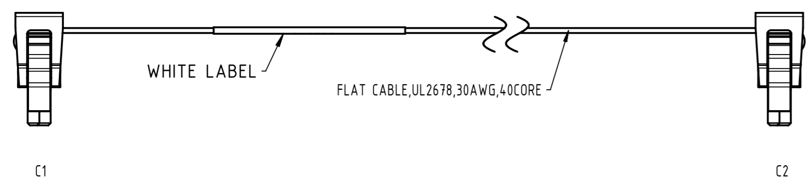
HAR-FLEX 40P Female With Strain Relief
